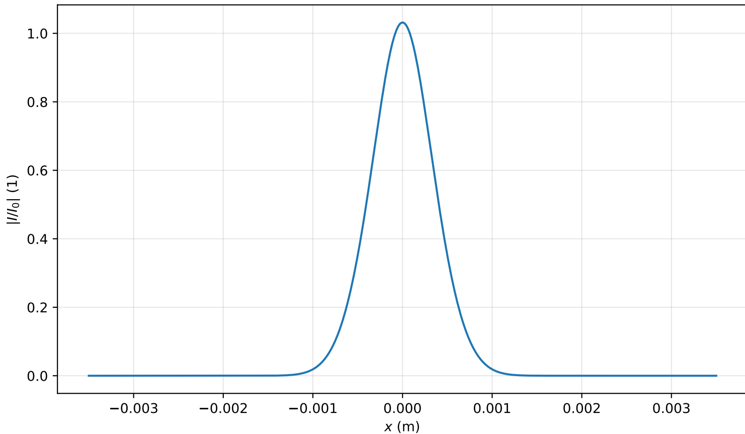
Intensity profile I(x, y = 0, z = 0.398m)/I_0 , \text{Pin}=0.5\text{Pcr} , artificial time
